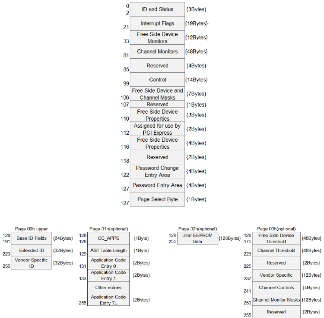
Figure 4 QSP28 Memory Map
