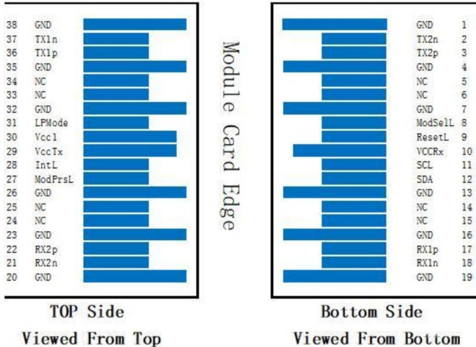
Figure 2 PIN MAP
